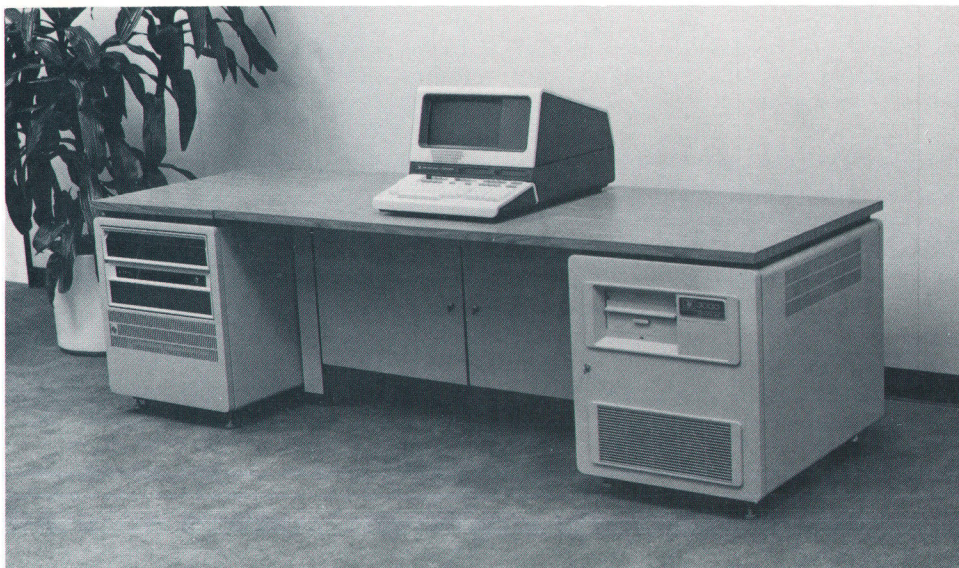
Fig. 1. HP 3000 Series 33 Computer System. Base model includes a 20M-byte cartridge disc drive, 256K bytes of fault-control memory, seven ports for 2400-baud asynchronous terminals, two general I/O channels, and a one-megabyte double-sided flexible disc drive. The Series 33 runs the same Multiprogramming Executive operating system (MPE III) as the more powerful HP 3000 Series II and Series III systems, and will execute Series II and Series III application programs without changes or recompilations.
